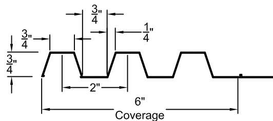
FORMLINER DETAIL
