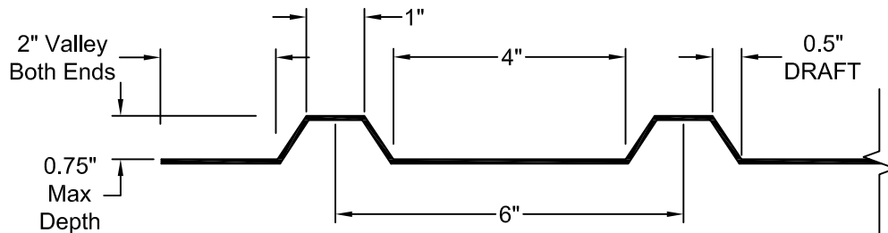
FORMLINER DETAIL
