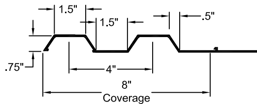
FORMLINER DETAIL
