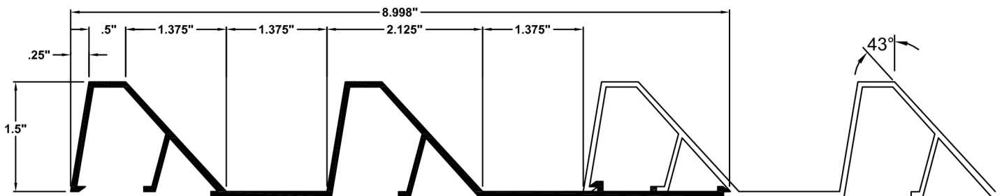
FORMLINER DETAIL
