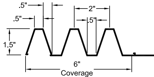
FORMLINER DETAIL
