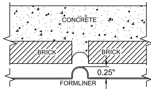
FORMLINER DETAIL
