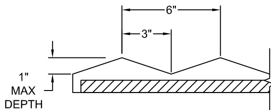
FORMLINER DETAIL
