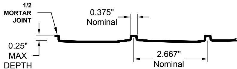
FORMLINER DETAIL
