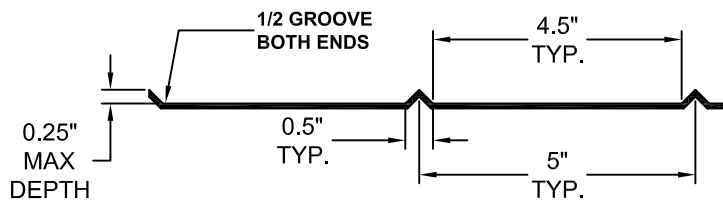
FORMLINER DETAIL
