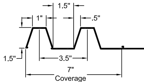
FORMLINER DETAIL
