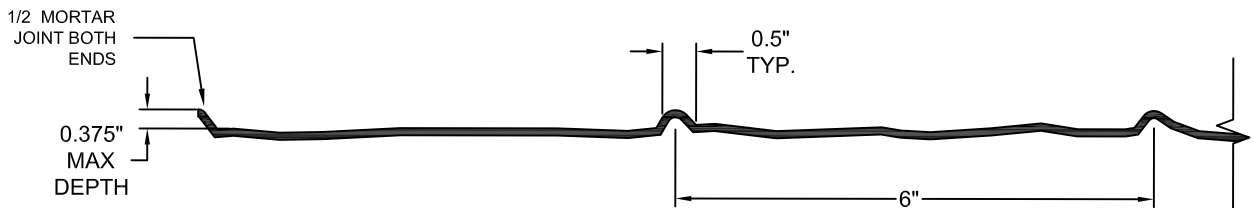
FORMLINER DETAIL
