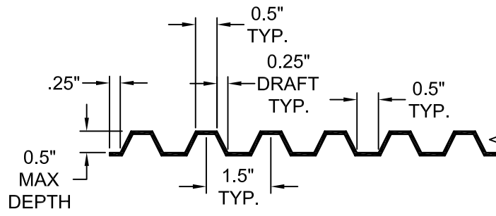
FORMLINER DETAIL
