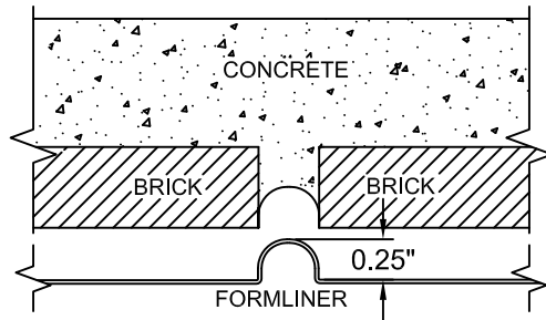
FORMLINER DETAIL
