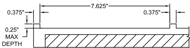
Detail A FORMLINER DETAIL
