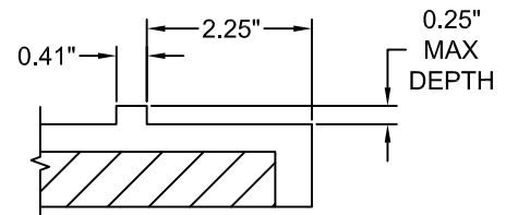
Detail B FORMLINER DETAIL
