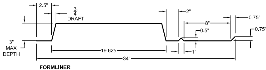
SECTION A-A FORMLINER DETAIL
