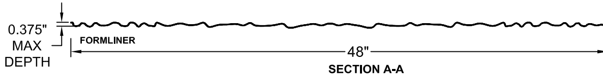
FORMLINER DETAIL
