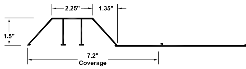
FORMLINER DETAIL
