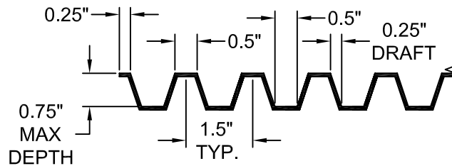
FORMLINER DETAIL
