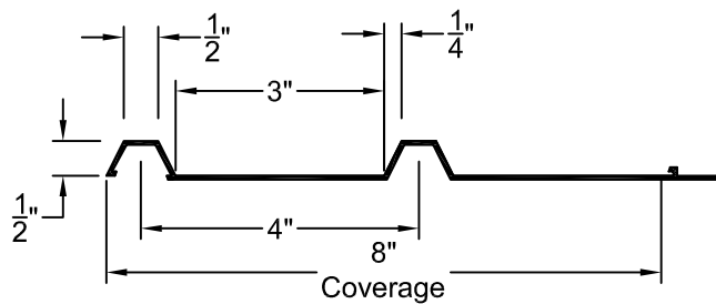
FORMLINER DETAIL
