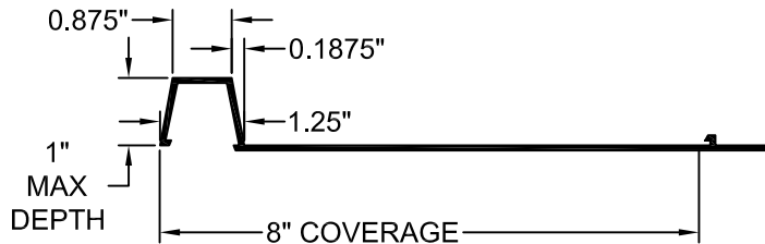
FORMLINER DETAIL
