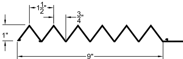
SECTION A-A FORMLINER DETAIL
