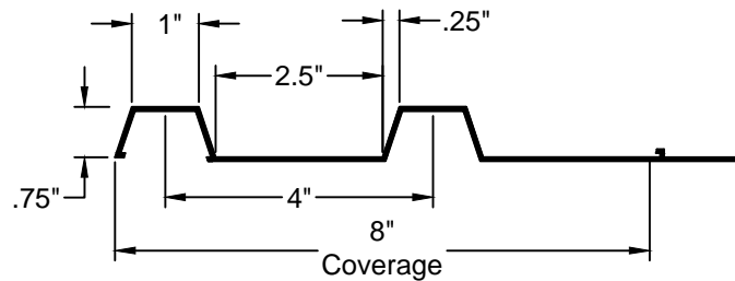
FORMLINER DETAIL
